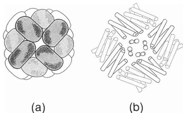
FIGURE 4 Schematic drawings of the subunit arrangement in an apo-ferritin molecule viewed down a fourfold axis (Banyard et al., 1978). (a) Complete molecular structure with a spherical shell of 24 polypeptide subunits. Centers of the quaternary structure are considered to be channels passing through the polypeptide shell which provide access routes for iron atoms forming an iron oxide core. Currently there is great interest in the structure and function of the outer shell itself, since the new application of ferritin has been reported as a reaction cavity for the preparation of inorganic nanometer particles (Meldrum et al., 1991). (b) Subunits related by a fourfold axis following the electron density map.
